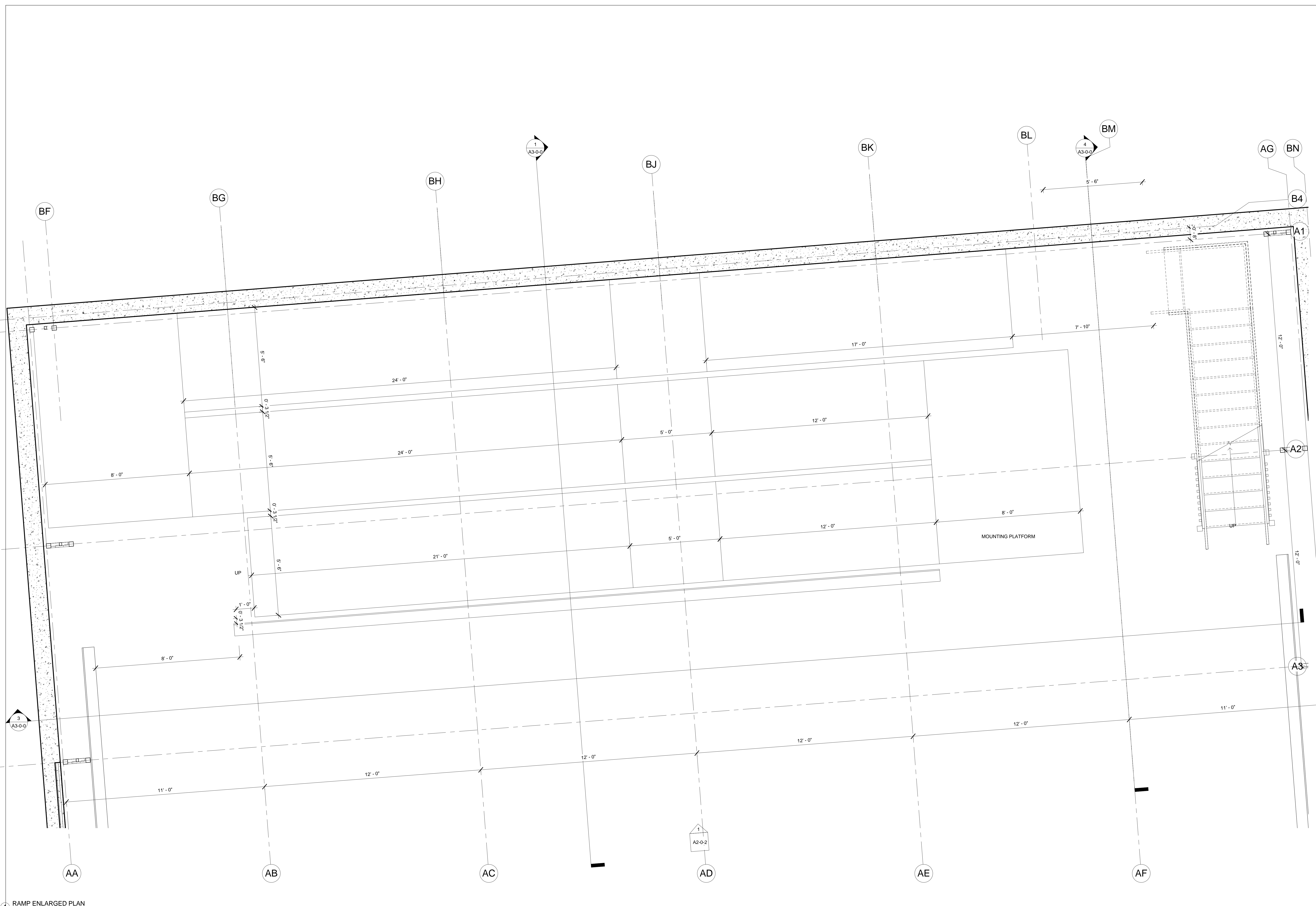
1 RAMP ENLARGED PLAN 1/2" = 1'-0"
